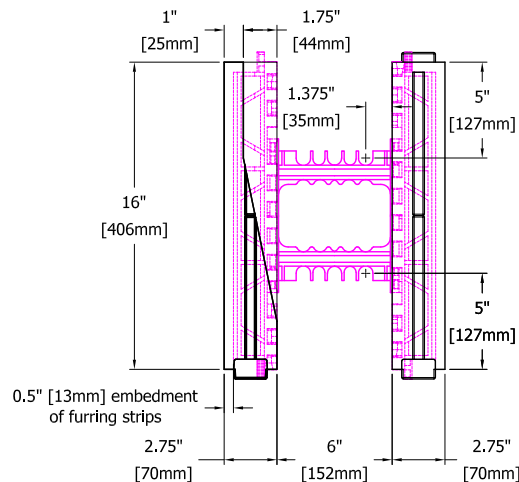
END VIEW
