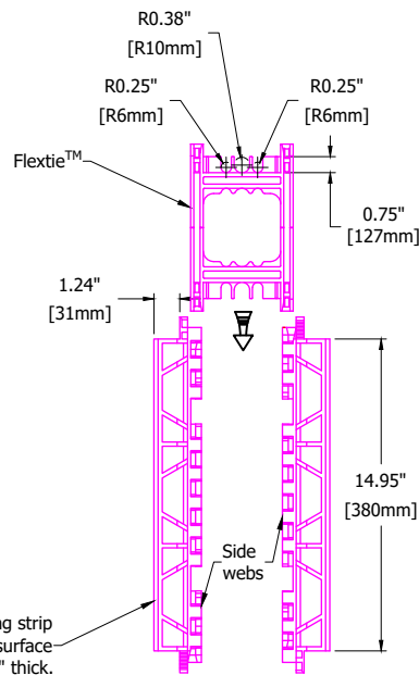
WEB TIE COMPONENTS
