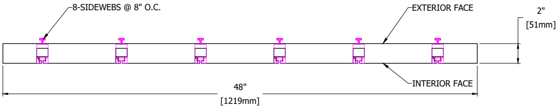
PLAN VIEW
