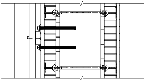
PLAN VIEW SHOWING EXPANSION ANCHORS ALONG SUBGIRT
