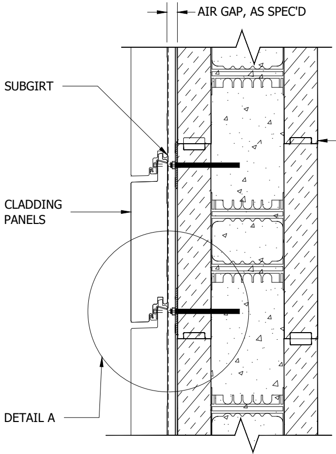
WALL SECTION ALONG SUBGIRTS
