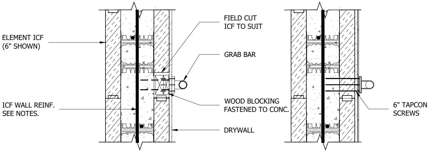
WOOD BLOCKING
