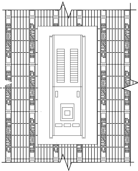
FRONT VIEW B-B
