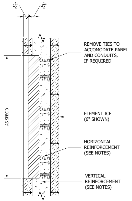
END VIEW A-A
