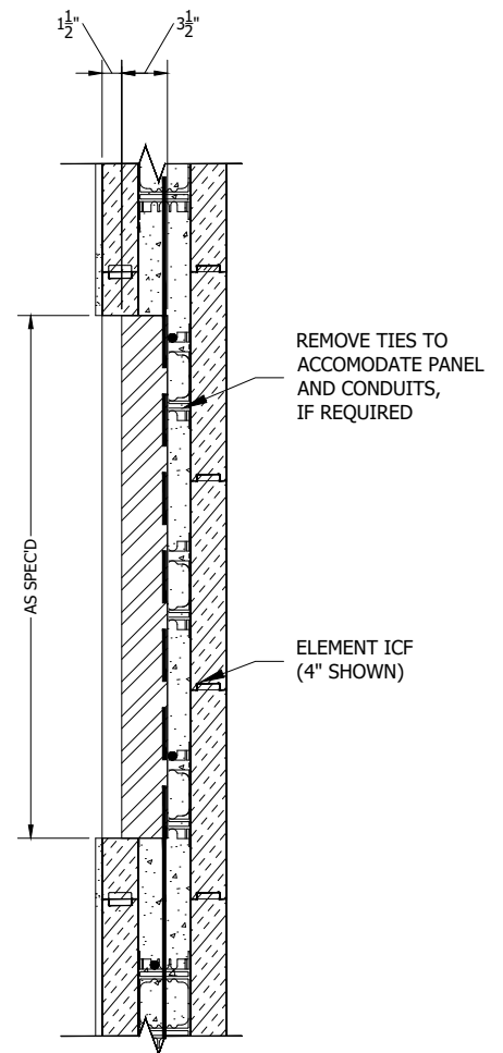
END VIEW A-A
