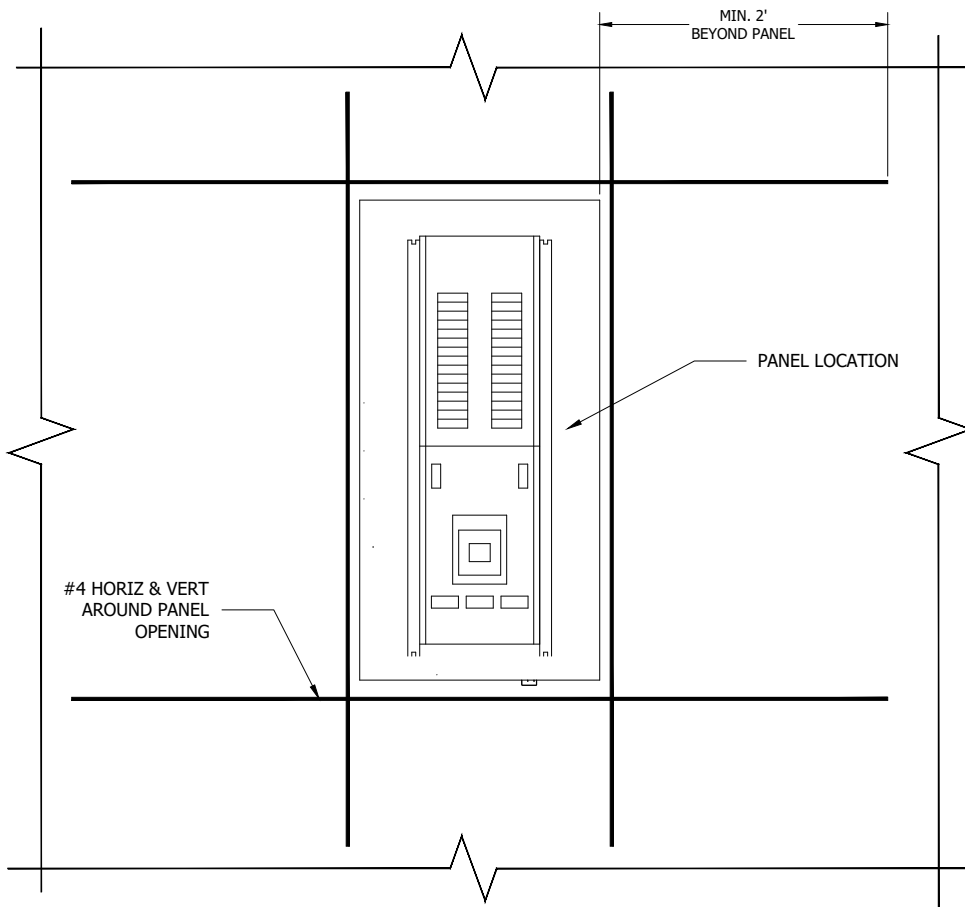
FRONT VIEW B-B
