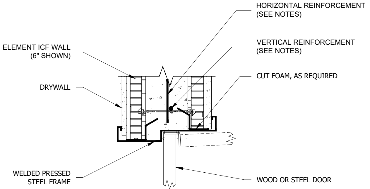
INTERIOR DOOR FRAME - JAMB CENTER MOUNTED DOOR
