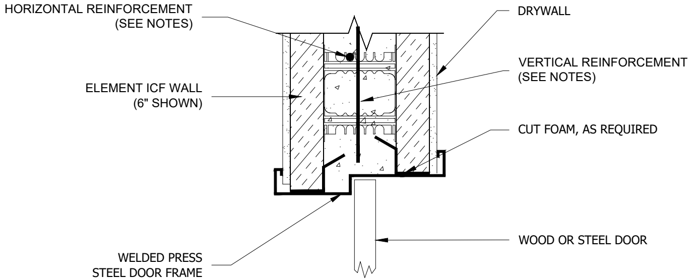
INTERIOR DOOR FRAME - HEAD CENTER MOUNTED DOOR
