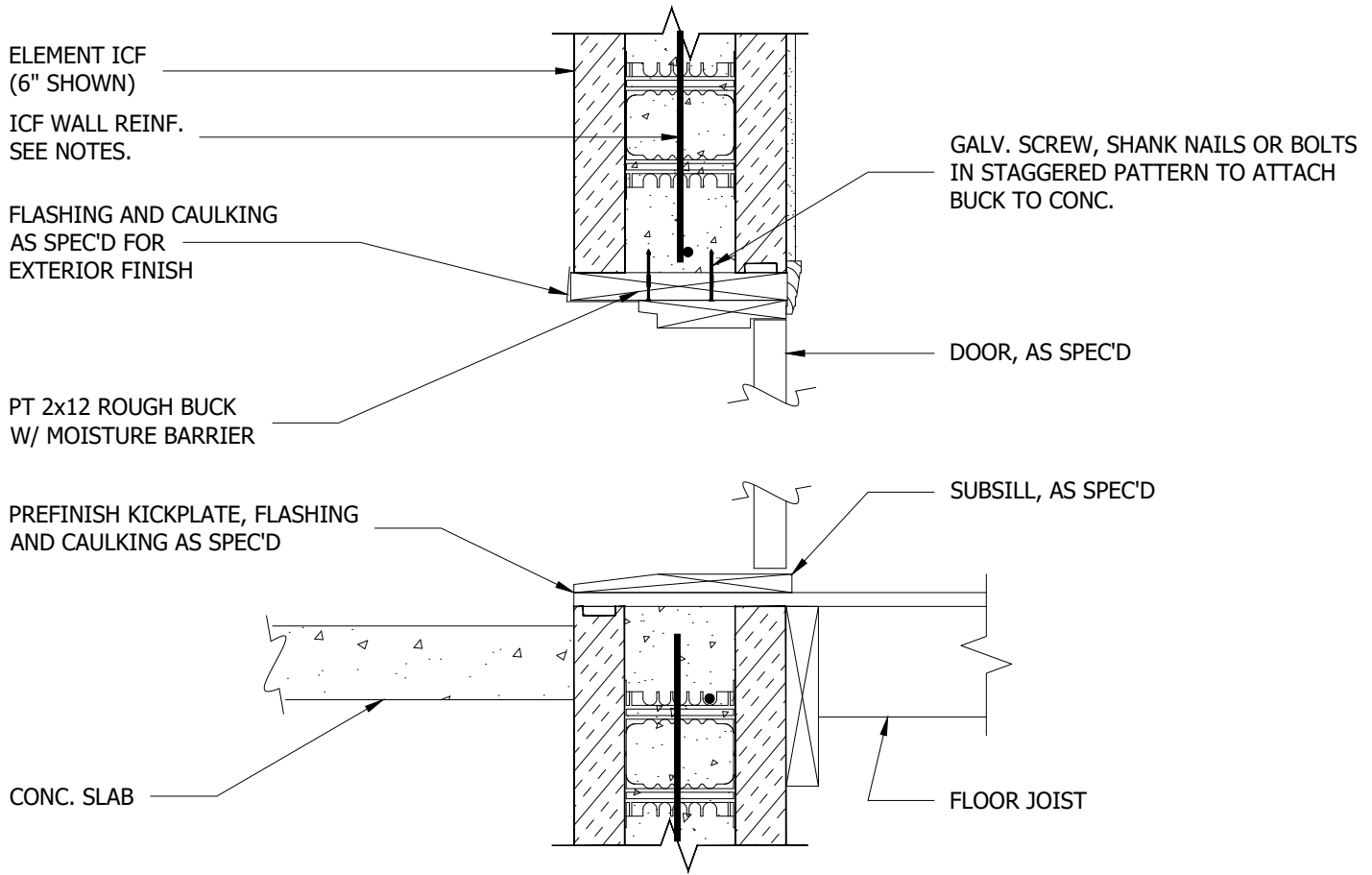
DOOR HEAD & SILL USING WOOD BUCKS
