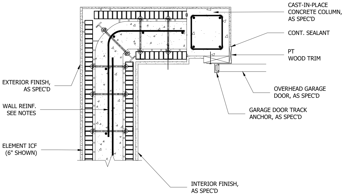
AGAINST CAST-IN-PLACE CONCRETE
