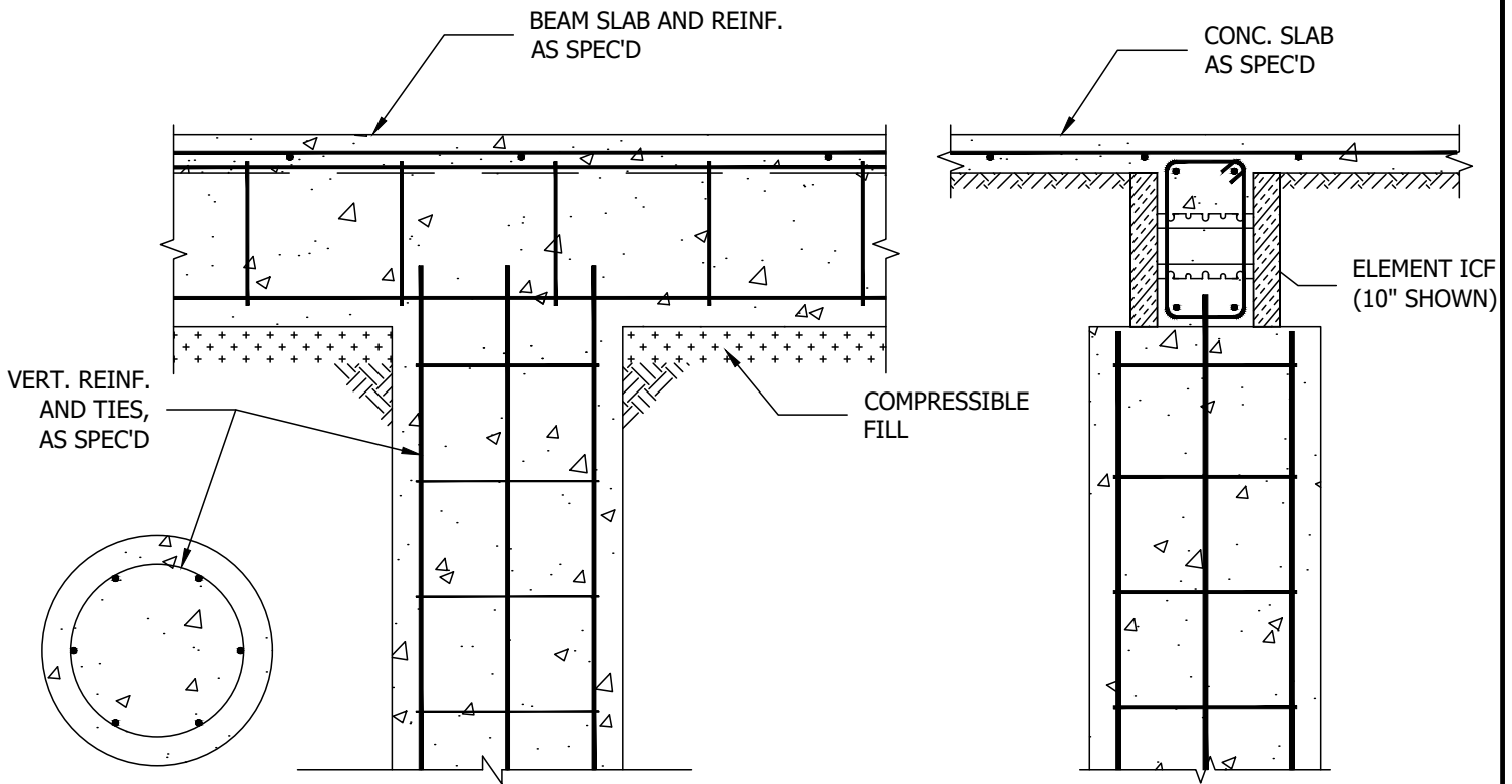
SIDE VIEW - Section through Grade Beam
