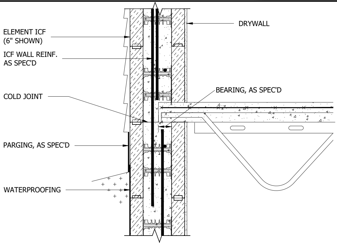
HAMBRO FLOOR SYSTEM (BEARING END)
