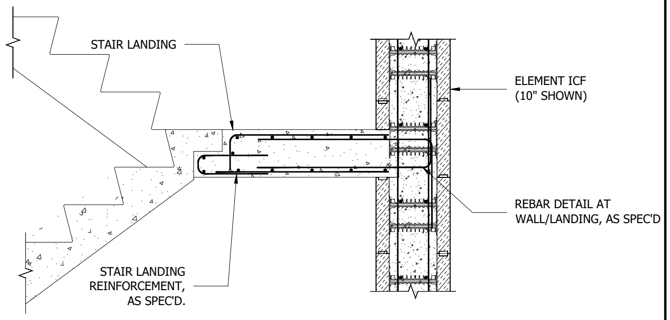
SECTION AT EXTERIOR WALL
