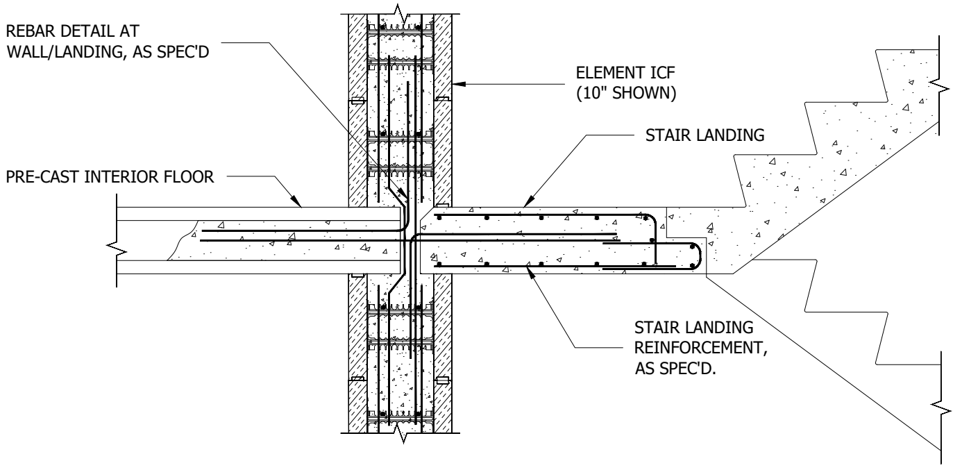
SECTION AT INTERIOR WALL
