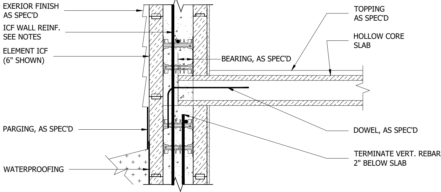
HOLLOW CORE PRECAST CONCRET SLAB (BEARING END)
