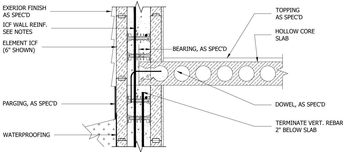
HOLLOW CORE PRECAST CONCRET SLAB (NON-BEARING END)
