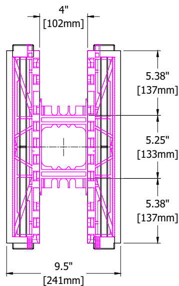
END VIEW SITE-ASSEMBLED BLOCK
