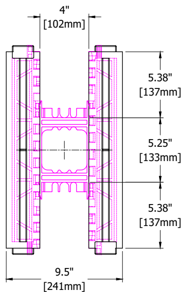
END VIEW SITE-ASSEMBLED BLOCK
