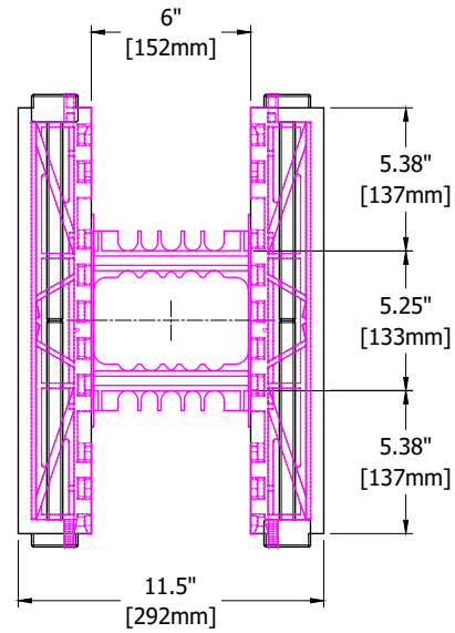
END VIEW SITE-ASSEMBLED BLOCK
