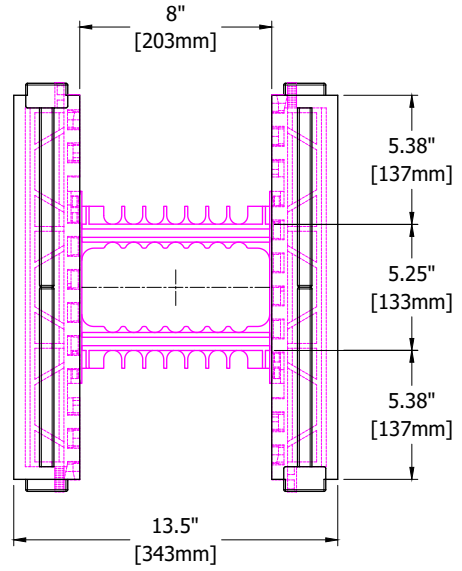
END VIEW SITE-ASSEMBLED BLOCK
