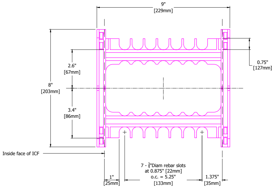
8 INCH FLEXTIE™
