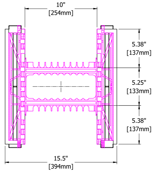
END VIEW SITE-ASSEMBLED BLOCK
