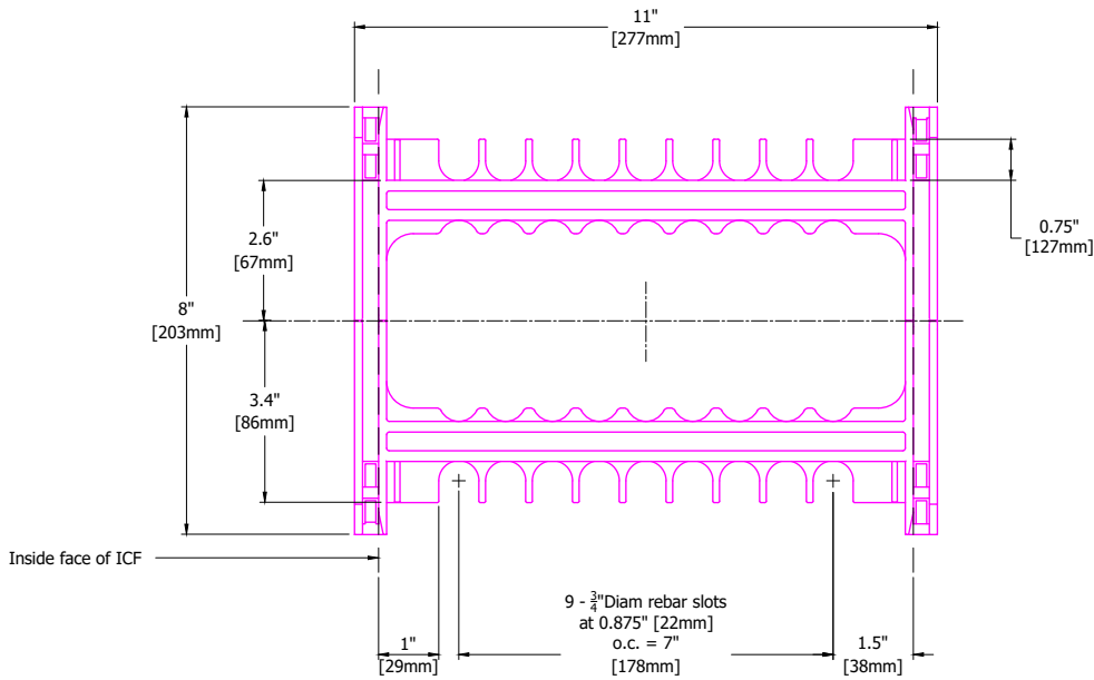
10 INCH FLEXTIE™
