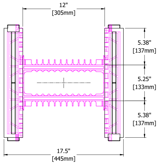
END VIEW SITE-ASSEMBLED BLOCK
