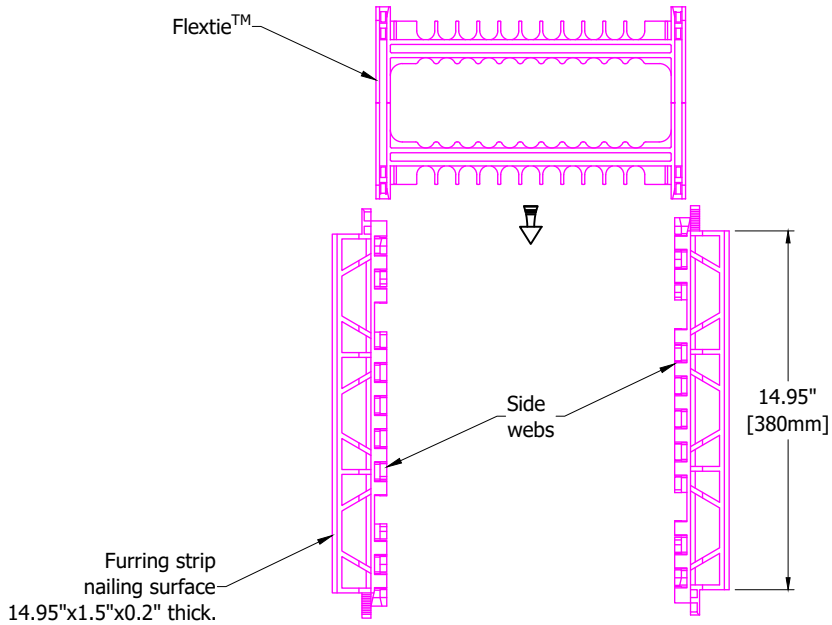
WEB TIE COMPONENTS
