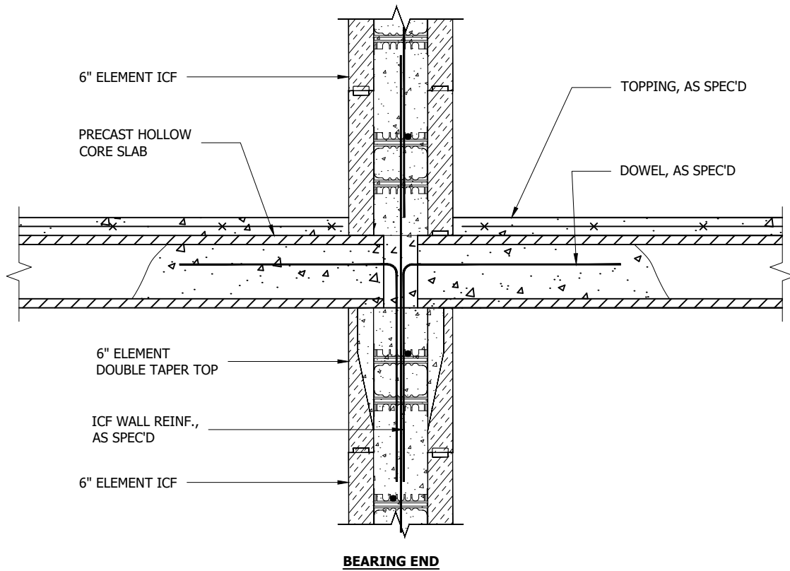
BEARING END
