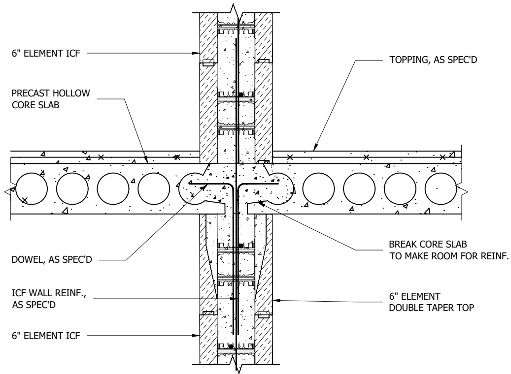
NON-BEARING END
