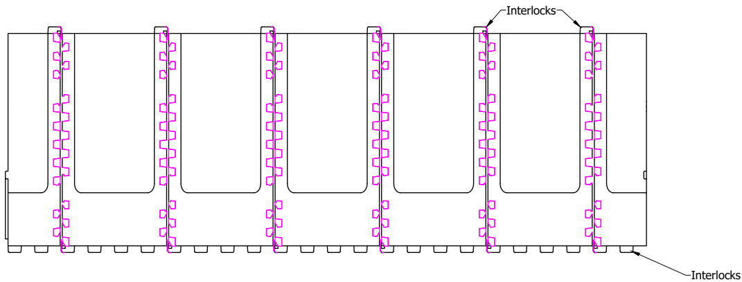
ELEVATION INTERIOR FACE
