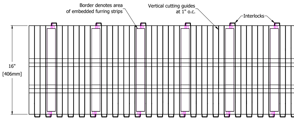
ELEVATION EXTERIOR FACE
