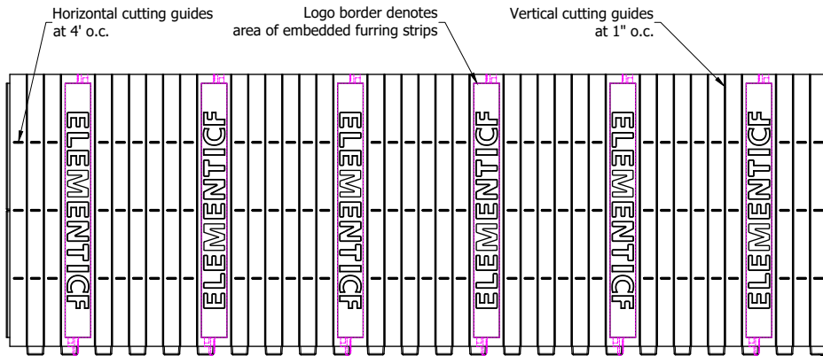
SIDE ELEVATION EXTERIOR FACE
